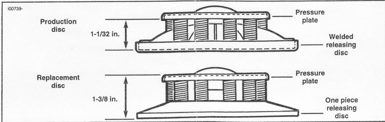
Pressure Plate to Releasing Disc Measurement
